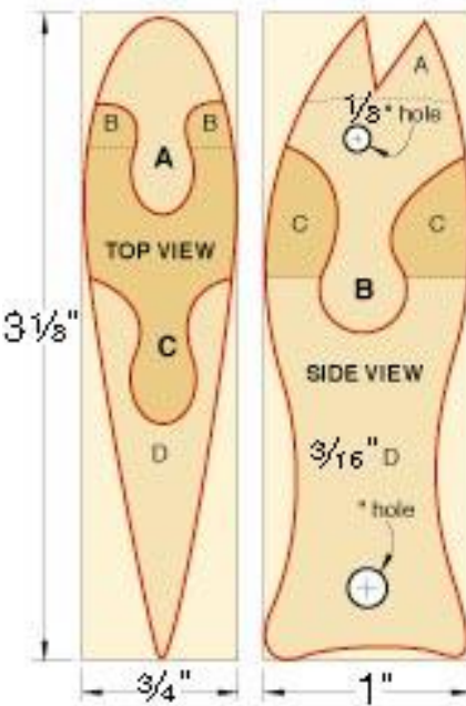
FISH KEY RING FULL-SIZE PATTERNS Red lines indicate bandsaw cuts
